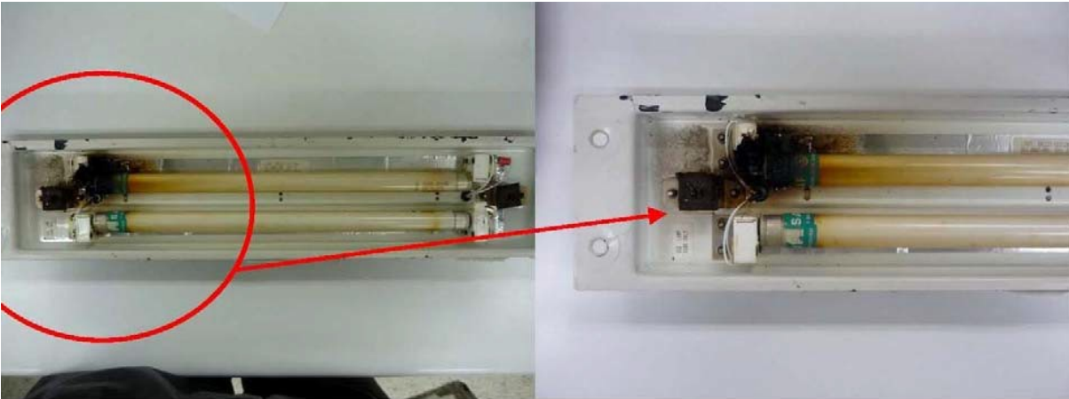
(MSN 29906) GALLEY 1 WORK LIGHT ASSY HOLDERS ARCED
